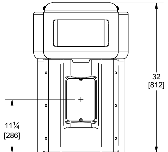
WITH 20" SHROUD
