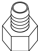
18615 3/4" NPT FEMALE TO 5/8" HB SWIVEL NYLON
